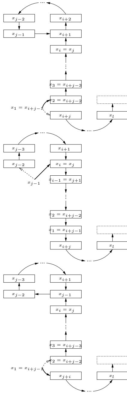
FIG. 2. Stages of an insertion of key x_1 , involving the movement of keys x_1, \dots, x_l . Boxes correspond to cells in either of the two tables, and arcs show possibilities for moving keys. A bold arc shows where the nestless key is to be inserted.
