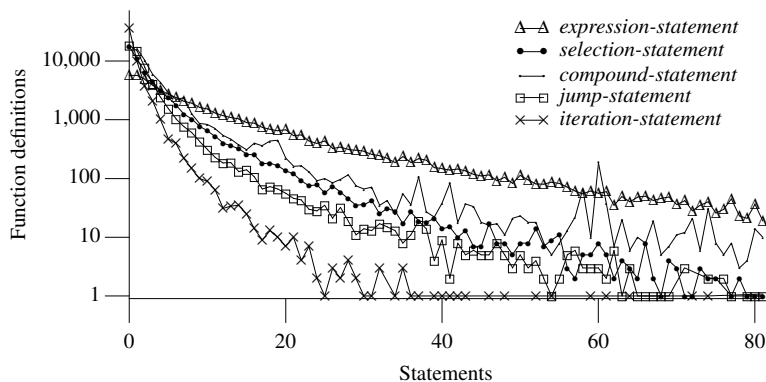
Figure 1696.9: Number of each kind of statement in function definitions. Based on the translated form of this book's benchmark programs.
