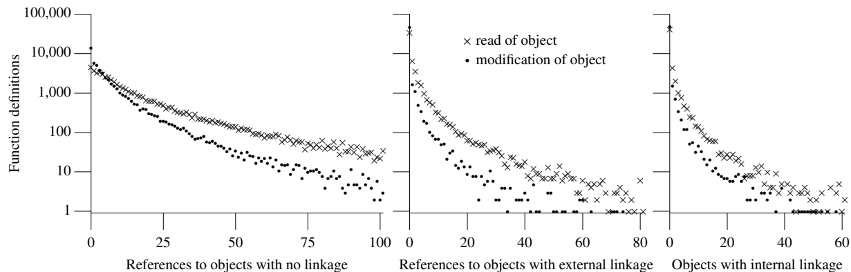
Figure 1805.5: Number of references (i.e., an access or modification) to all objects, having various kinds of linkage, within individual function definitions. Based on the translated form of this book's benchmark programs.
