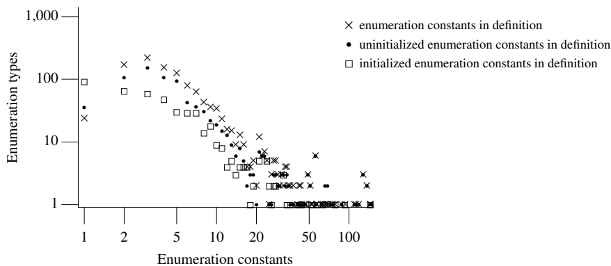
Figure 1430.1: Number of enumeration constants in an enumeration type and number whose value is explicitly or implicitly specified. Based on the translated form of this book's benchmark programs (also see Figure 295.1).
