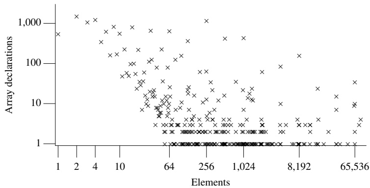
Figure 524.1: Number of arrays defined to have the given number of elements. Based on the translated form of this book’s benchmark programs.
