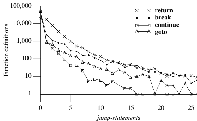
Figure 1768.1: Number of function definitions containing a given number of jump-statements . Based on the translated form of this book's benchmark programs.
