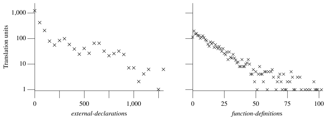
Figure 1794.1: Number of external-declarations and function-definitions declared during the translation of this book's benchmark programs (rounded to the nearest fifty and excluding identifiers declared in any system headers that are #included ).
