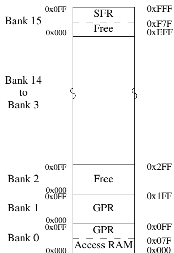
Figure 555.1: Data storage organization for the PIC18CXX2 devices [895] The 4,096 bytes of storage can be treated as a linear array or as 16 banks of 256 bytes (different instructions and performance penalties are involved). Some storage locations hold Special Function Registers (SFR) or General Purpose Registers (GPR). Free denotes storage that does not have a preassigned usage and is available for general program use.
