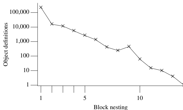
Figure 405.1: Number of object declarations appearing at various block nesting levels (level 1 is the outermost block). Based on the translated form of this book's benchmark programs.
