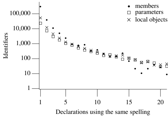
Figure 394.2: Number of declarations of an identifier with the same spelling in the same translation unit. Based on the translated form of this book’s benchmark programs. Note that members of the same type are likely to be counted more than once (i.e., they are counted in every translation unit that declares them), while parameters and objects declared within function definitions are likely to be counted once.
