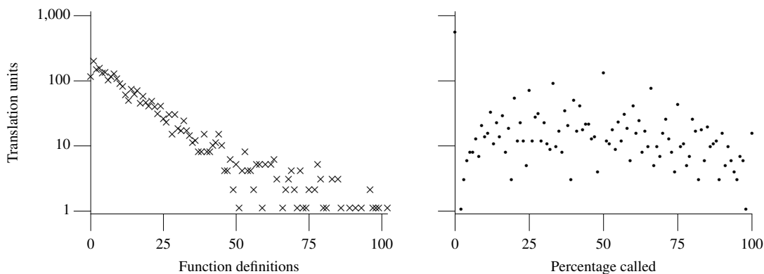
Figure 1794.2: Number of functions defined in each translation unit and percentage of functions that are called within the translation unit that defines them. Based on the translated form of this book's benchmark programs.
