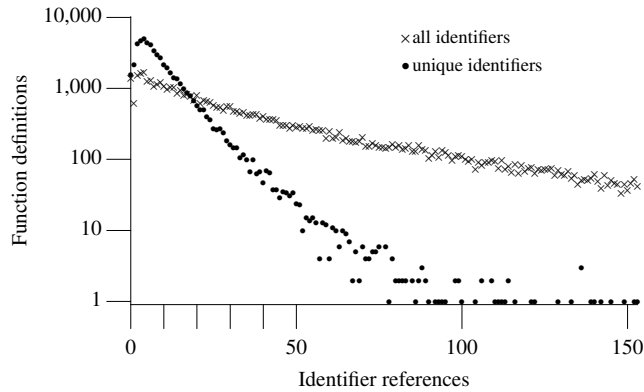
Figure 787.25: Number of identifiers referenced within individual function definitions. Based on the translated form of this book's benchmark programs.
