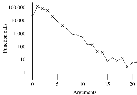
Figure 286.1: Number of arguments passed in function calls. Based on the translated form of this book's benchmark programs.
