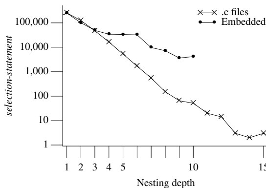
Figure 1728.2: Number of selection-statements having a given maximum nesting level for embedded C [376] (whose data was multiplied by a constant to allow comparison; the data for nesting depth 5 was interpolated) and the visible form of the .c files.
