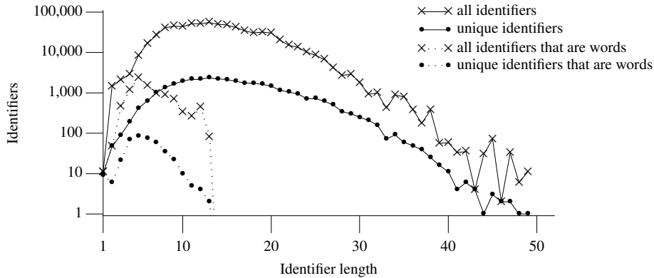
Figure 280.1: Number of identifiers, with external linkage, having a given length, based on the translated form of this book's benchmark programs. Information on the length of all identifiers in the visible source is given elsewhere (see Figure 787.7).
