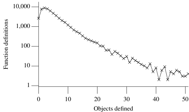
Figure 283.1: Number of declarations of identifiers as objects within all of the blocks contained in a function definition. Based on the translated form of this book’s benchmark programs.
