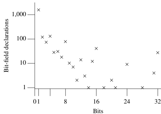
Figure 1383.1: Number of bit-field declarations specifying the given number of bits. Based on the translated form of this book's benchmark programs. (Declarations encountered in any source or header file were only counted once, the contents of system headers were ignored.)
