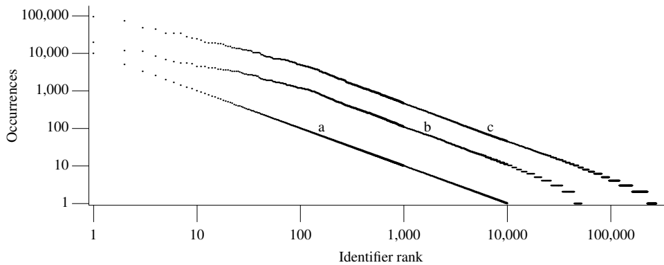
Figure 787.26: Identifier rank (based on frequency of occurrence of identifiers having a particular spelling) plotted against the number of occurrences of the identifier in the visible source of (b) Mozilla, and (c) Linux 2.4 kernel; (a) is a distribution following Zipf's law with the most common item occurring 10,000 times. Every identifier is represented by a dot.
