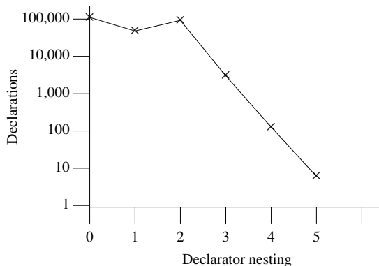
Figure 276.1: Number of full declarators containing a given number of modifiers, based on the translated form of this book’s benchmark programs.
