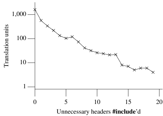
Figure 1877.1: Number of #include s of header-names whose contents are not referenced during translation. Based on the translated form of this book's benchmark programs.
