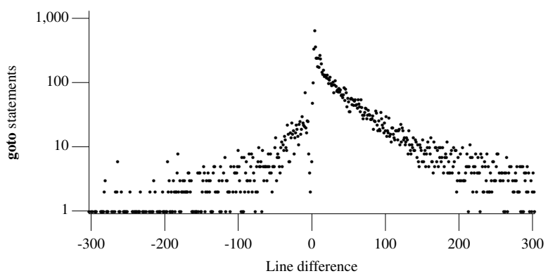
Figure 1769.1: Number of visible source lines between a goto statement and its destination label (negative values denote backward jumps). Based on the translated form of this book’s benchmark programs.
