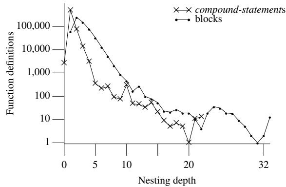
Figure 274.1: Maximum nesting of blocks and compound-statements within function definitions, based on the visible form of the .c files.
