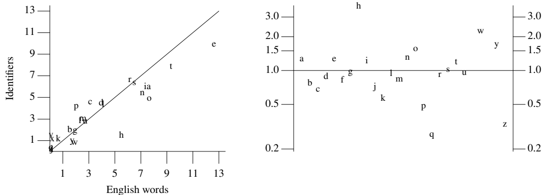
Figure 787.16: Occurrence of alphabetic letters in English text [1212] and identifier names (based on the visible form of the .c files; all letters mapped to lowercase). Left graph plots the letter percentage occurrence as (x, y) coordinates and right graph plots the ratio of dividing the English by the identifier letter frequency (i.e., letters above the line are more common in English text than in identifiers; two letters outside the range plotted are v = 0.0588 and x = 0.165 ).
