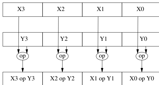
Figure 1368.1: Behavior of packed single-precision floating-point operations supported by the Intel Pentium processor. [607]
