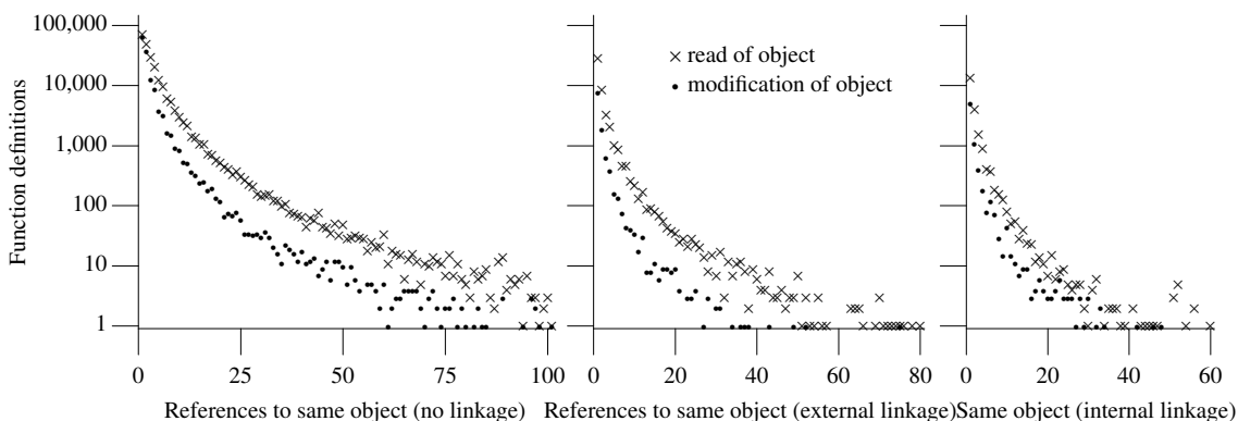
Figure 1805.6: Number of references (i.e., an access or modification) to the same object, having various kinds of linkage, within individual function definitions. Based on the translated form of this book's benchmark programs.
