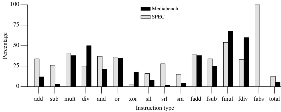
Figure 0.3: Percentage of trivial computations during program execution of the SPEC and MediaBench benchmarks for various kinds of operation. Adapted from Yi and Lilja. [1423]
