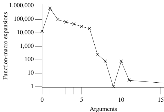
Figure 288.1: Number of arguments in expansions of function-like macros, excluding expansions that occurred while processing system headers, during translation of this book's benchmark programs.
