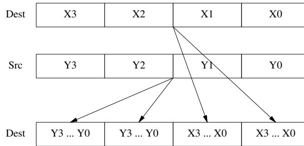
Figure 933.1: The SHUFPS (shuffle packed single-precision floating-point values) instruction, supported by the Intel Pentium processor, [607] places any two of the four packed floating-point values from the destination operand into the two low-order doublewords of the destination operand, and places any two of the four packed floating-point values from the source operand into the two high-order doublewords of the destination operand. By using the same register for the destination and destination operands, the SHUFPS instruction can shuffle four single-precision floating-point values into any order.
