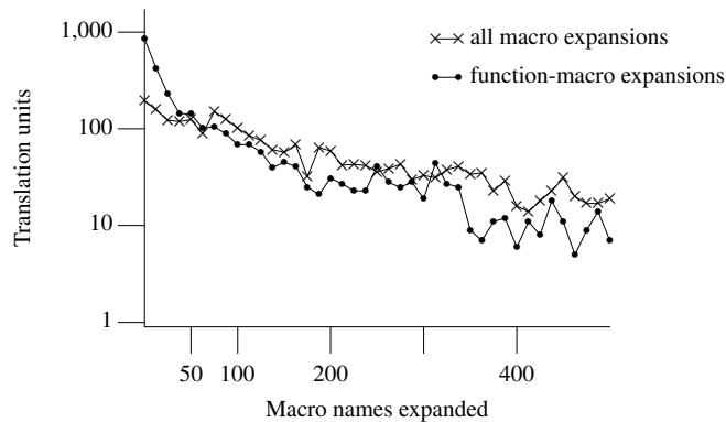
Figure 1912.1: Number of macro names expanded, excluding expansions occurring while processing the contents of system headers, during translation of this book's benchmark programs.
