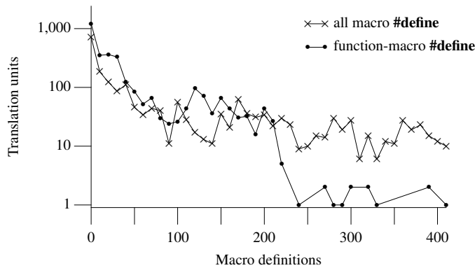
Figure 284.2: Number of #define directives evaluated in each translation unit, excluding the contents of system headers, during translation of this book’s benchmark programs (there were a total of 1,432,735 macros defined, of which 313,620 were function-like macros).
