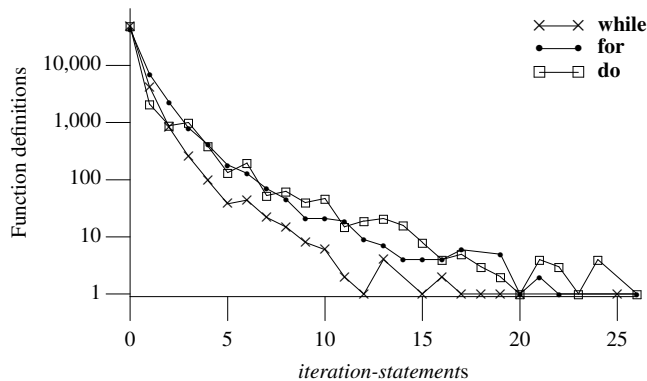
Figure 1752.1: Number of function definitions containing the given number of iteration-statements . Based on the translated form of this book's benchmark programs.
