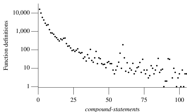
Figure 1699.1: Number of compound-statements in function definitions. Based on the translated form of this book's benchmark programs.
