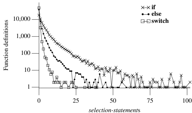
Figure 1728.1: Number of functions containing a given number of selection-statements . Based on the translated form of this book's benchmark programs.
