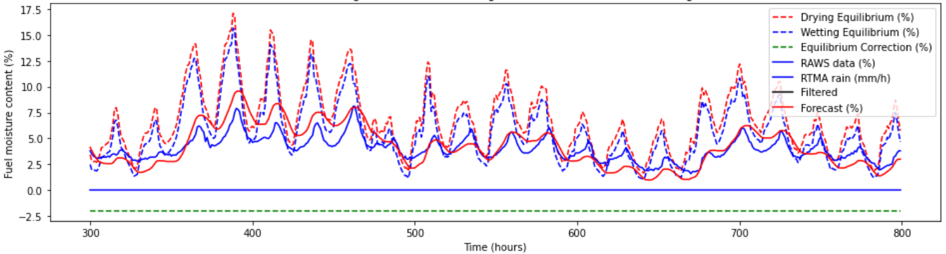
BKCU1 Kalman filtering and forecast with augmented state, real data. Training 0:300 hmax
